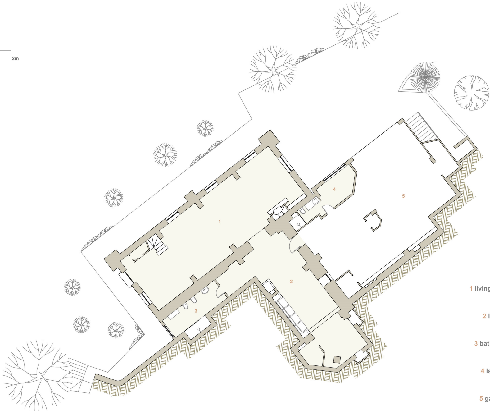
BASAMENT FLOOR
